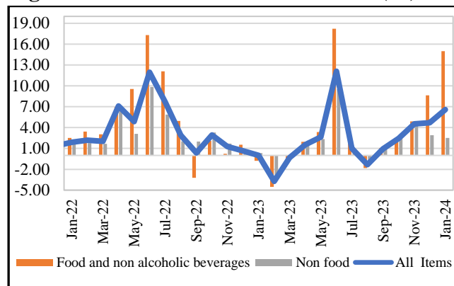
Figure 17: Month-on-Month Inflation (%)
